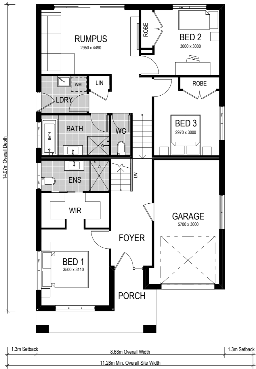
Lower Floor Bedroom Level
